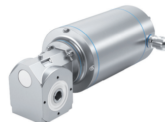
Worm gearbox SMN with stainless steel motor SBH with IP69K
